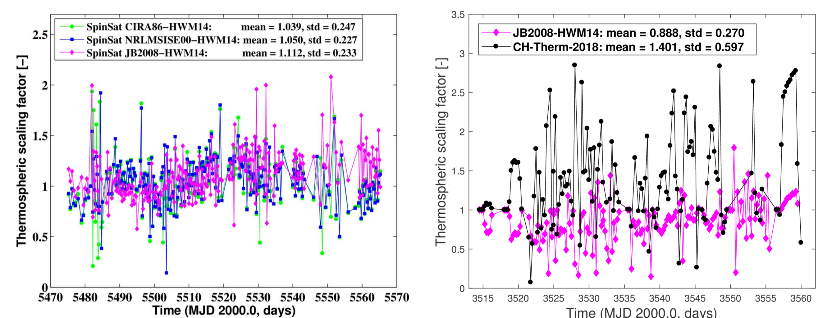
Figure 3: Scaling factor f_s estimated from SLR observations to SpinSat from 29 December 2014 to 29 March 2015 (left) and to ANDE-P from 16 August 2009 to 30 September 2009 (right).
