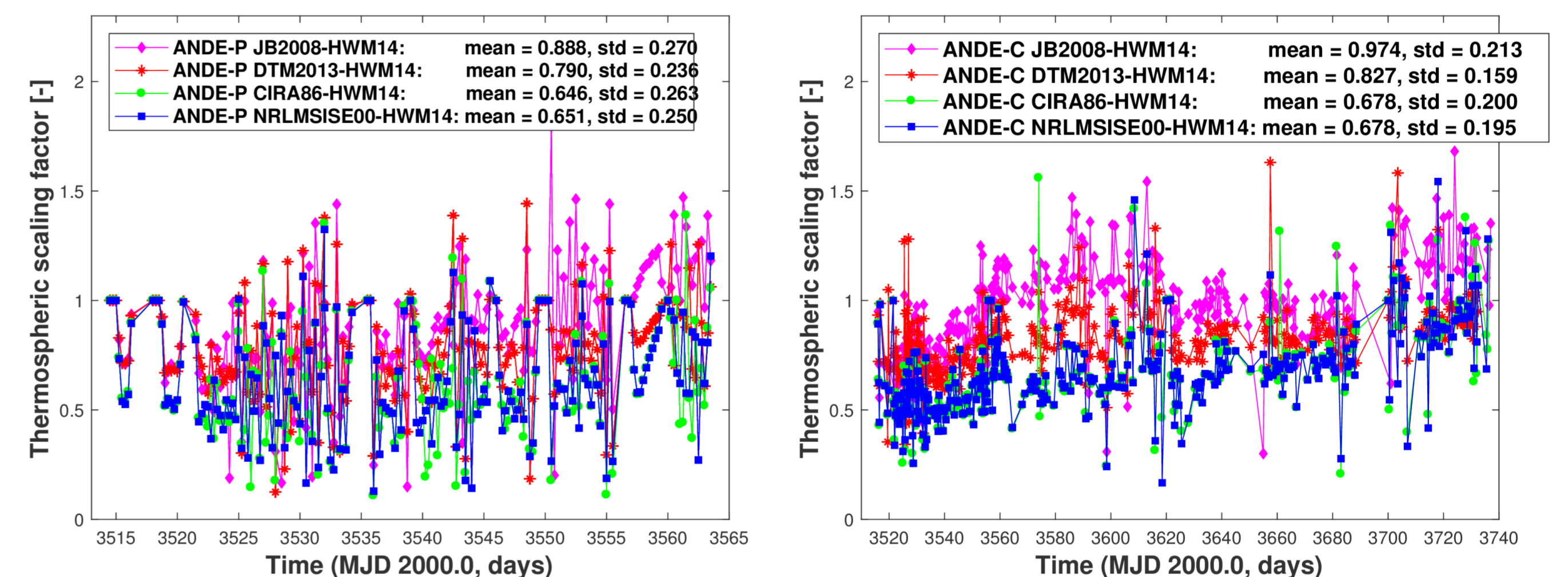
Figure 2: Scaling factor f_s estimated from SLR observations to ANDE-P from 16 August 2009 to 3 October 2009 (left) and to ANDE-C from 16 August 2009 to 26 March 2010 (right). The ANDE-C data analysis indicates a trend.
