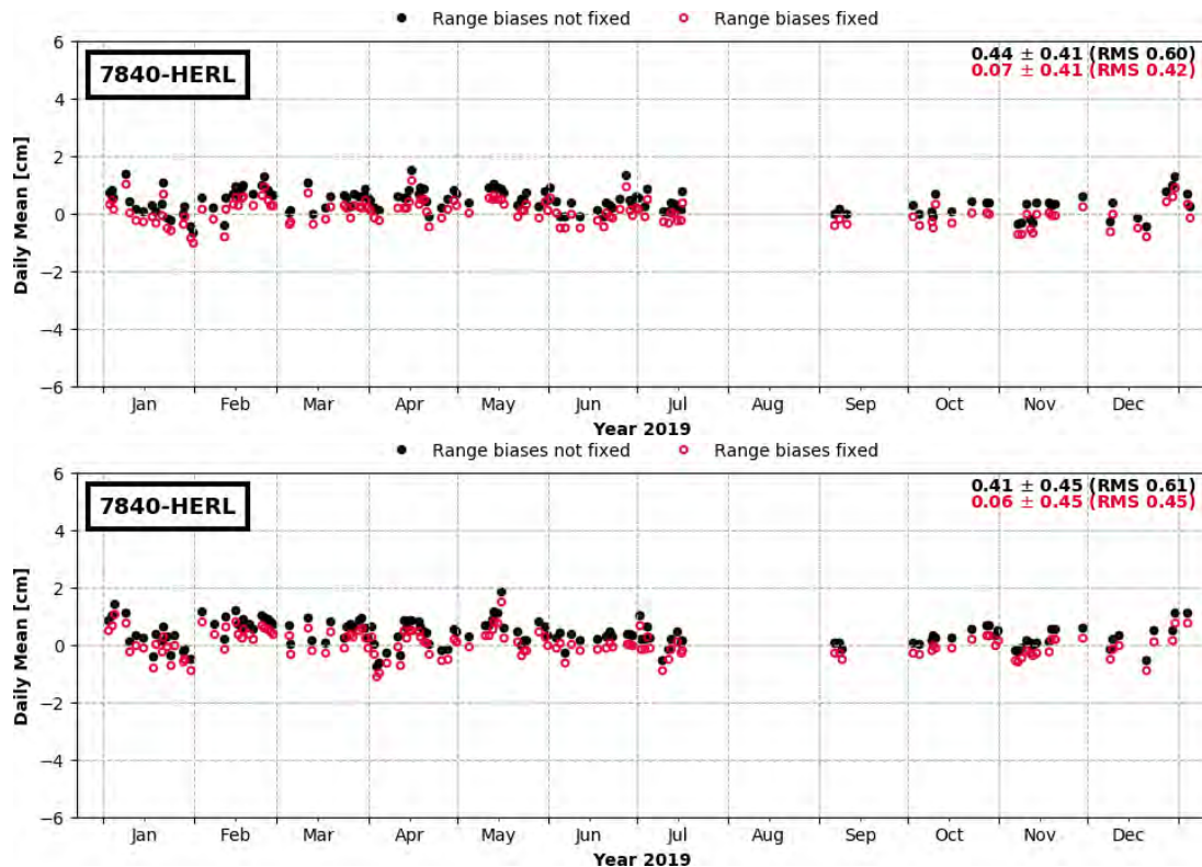
Figure 4-112: Daily mean of the SLR observation residuals [1-range; cm] of the SLR station 7840 (HERL) in 2019 (above Sentinel-3A, and below Sentinel-3B)
