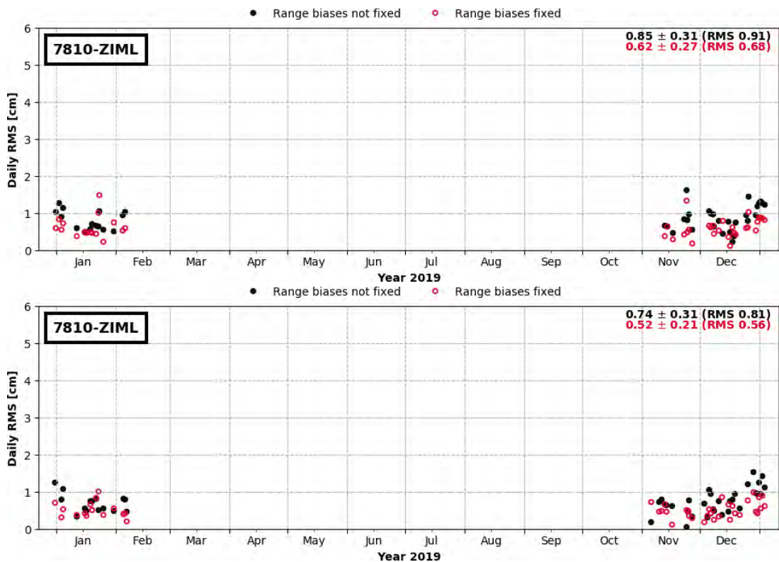
Figure 4-84: Daily RMS of the SLR observation residuals [1-range; cm] of the SLR station 7810 (ZIML) in 2019 (above Sentinel-3A, and below Sentinel-3B)
