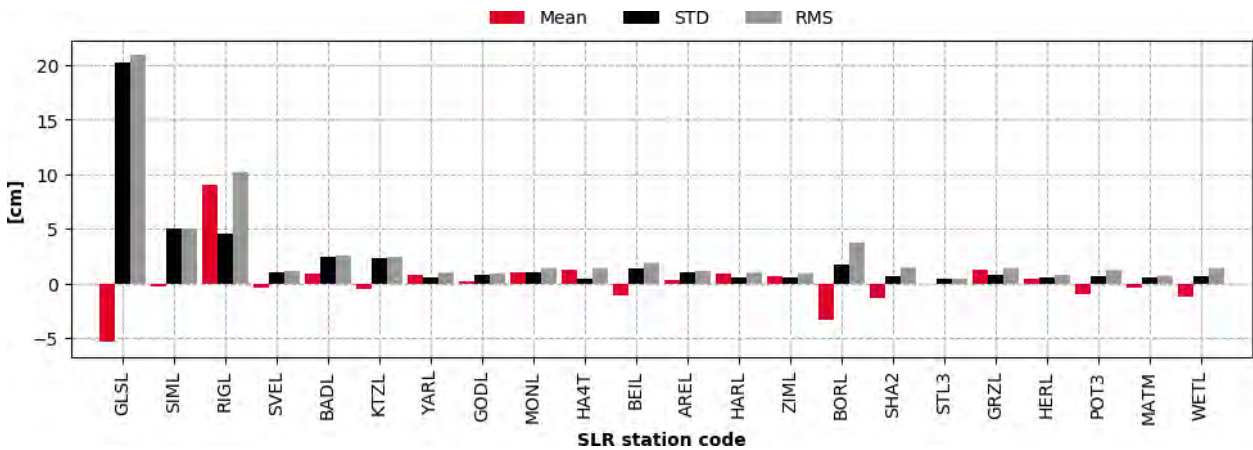
Figure 4-138: Mean, STD and RMS of the Sentinel-3A SLR observation residuals [1-range; cm] per each SLR station in 2019 (the range biases have been fixed) (the figure below is a zoomed-in of the figure above)
