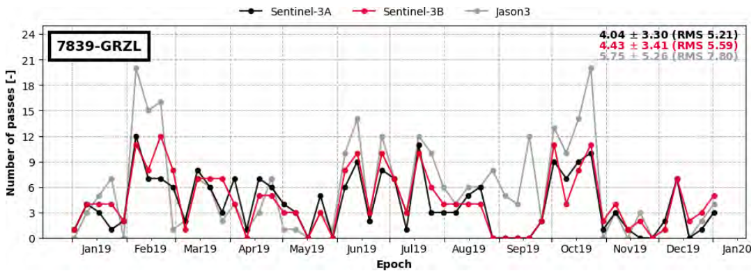
Figure 4-104: Total number of satellite passes per GPS week of the SLR station 7839 (GRZL) in 2019 (Sentinel-3A, Sentinel-3B and Jason-3)
