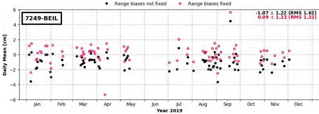
Figure 4-64: Daily mean of the SLR observation residuals [1-range; cm] of the SLR station 7249 (BEIL) in 2019 (above Sentinel-3A, and below Sentinel-3B)
