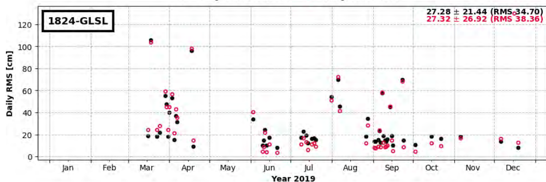
Figure 4-6: Daily RMS of the SLR observation residuals [1-range; cm] of the SLR station 1824 (GLSL) in 2019 (above Sentinel-3A, and below Sentinel-3B)
