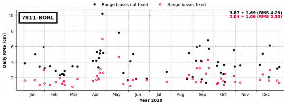
Figure 4-89: Daily STD of the SLR observation residuals [1-range; cm] of the SLR station 7811 (BORL) in 2019 (above Sentinel-3A, and below Sentinel-3B)
