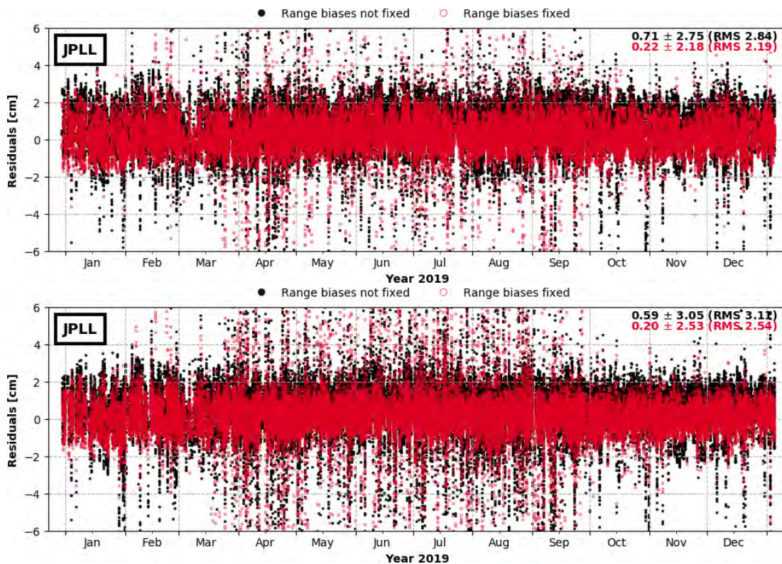
Figure 3-21: SLR observation residuals [1-range; cm] obtained for JPLL orbit solution in 2019 (above Sentinel-3A, and below Sentinel-3B)
