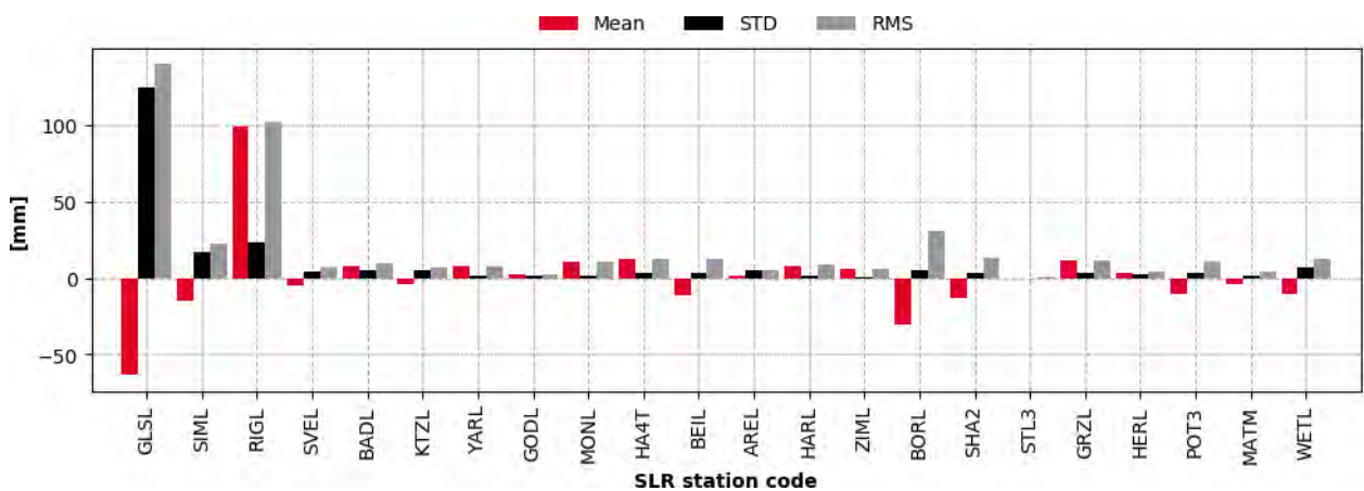
Figure 3-7: Mean, STD and RMS of the Sentinel-3A range biases [1-range; mm] of each SLR station (the figure below is a zoomed-in of the figure above)
