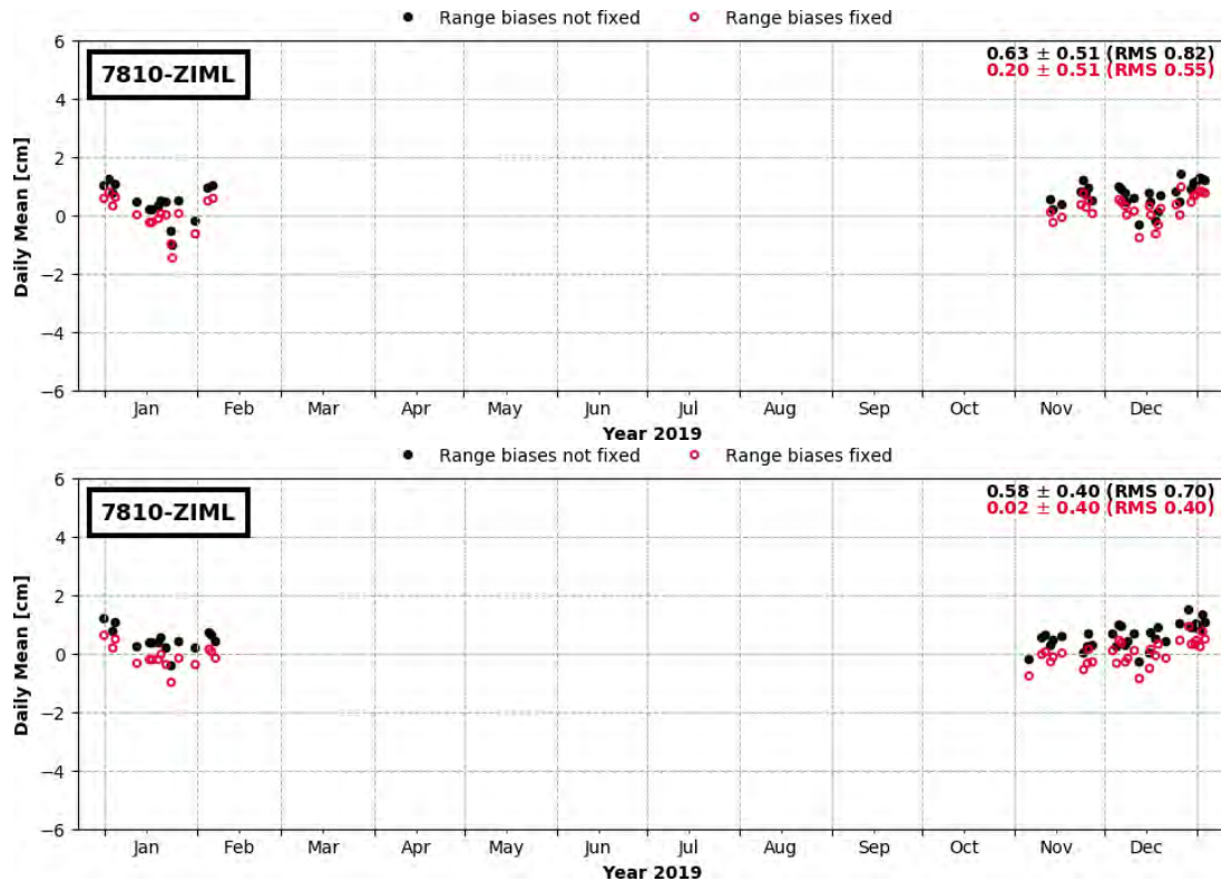
Figure 4-82: Daily mean of the SLR observation residuals [1-range; cm] of the SLR station 7810 (ZIML) in 2019 (above Sentinel-3A, and below Sentinel-3B)
