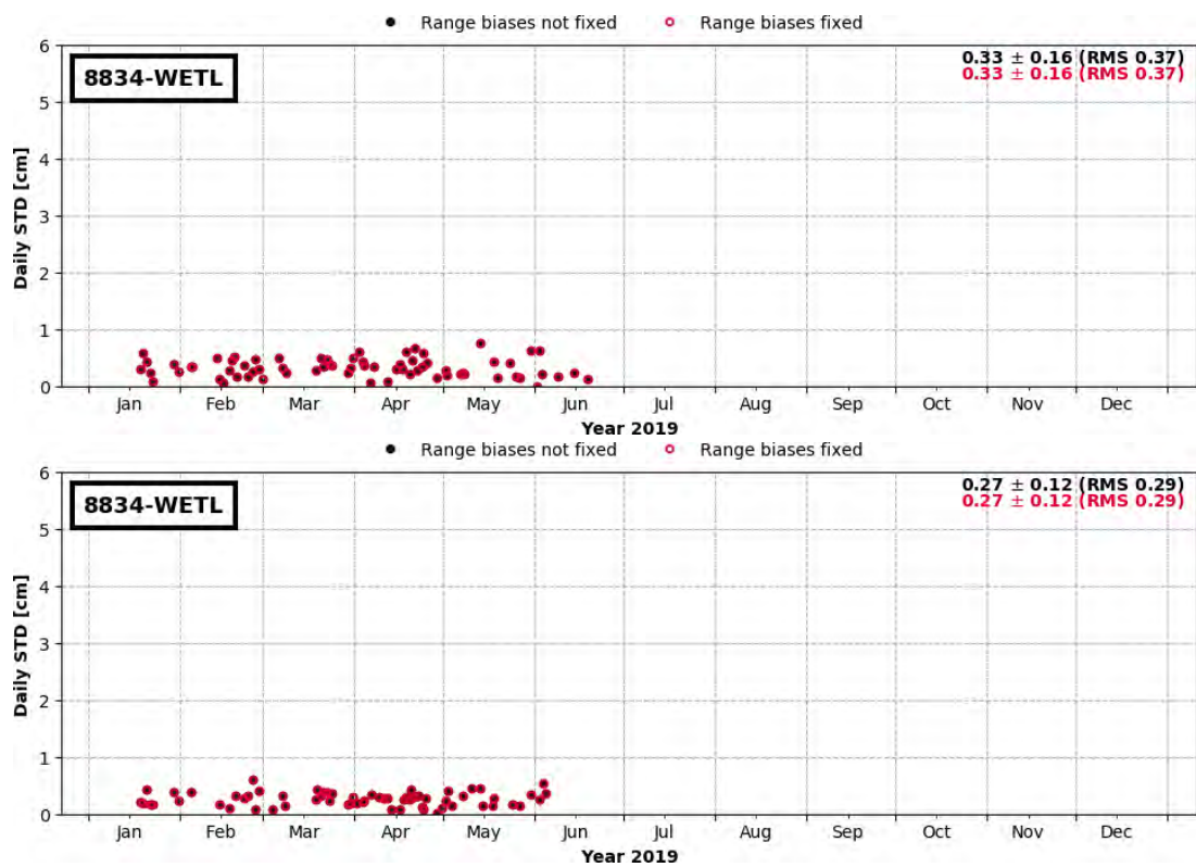
Figure 4-131: Daily STD of the SLR observation residuals [1-range; cm] of the SLR station 8834 (WETL) in 2019 (above Sentinel-3A, and below Sentinel-3B)
