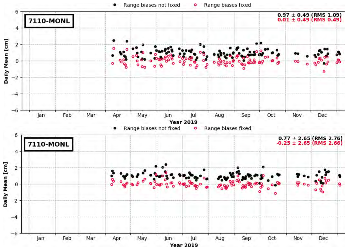
Figure 4-52: Daily mean of the SLR observation residuals [1-range; cm] of the SLR station 7110 (MONL) in 2019 (above Sentinel-3A, and below Sentinel-3B)
