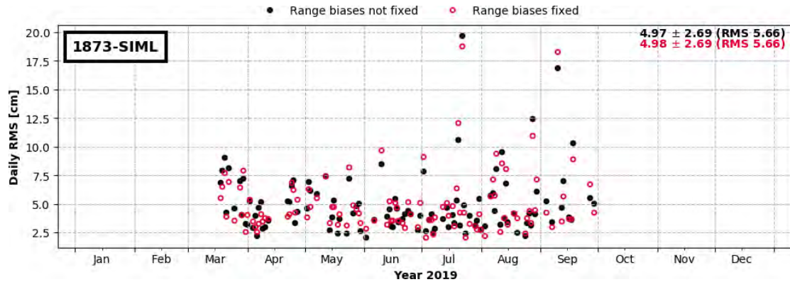
Figure 4-12: Daily RMS of the SLR observation residuals [1-range; cm] of the SLR station 1873 (SIML) in 2019 (only Sentinel-3B)
