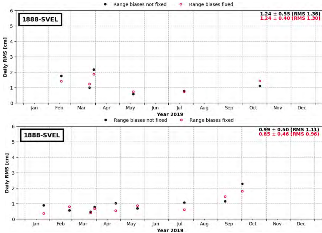
Figure 4-24: Daily RMS of the SLR observation residuals [1-range; cm] of the SLR station 1888 (SVEL) in 2019 (above Sentinel-3A, and below Sentinel-3B)
