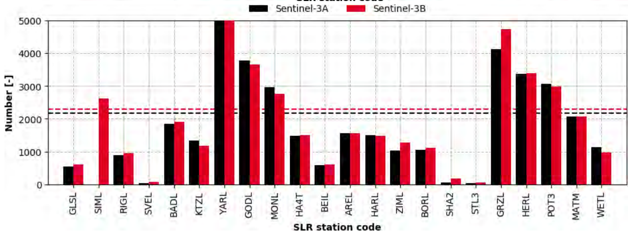
Figure 4-134: Total number of the SLR observations processed for Sentinel-3A and Sentinel-3B in 2019 (the figure below is a zoomed-in of the figure above) (the horizontal lines address the mean value for all SLR stations)
