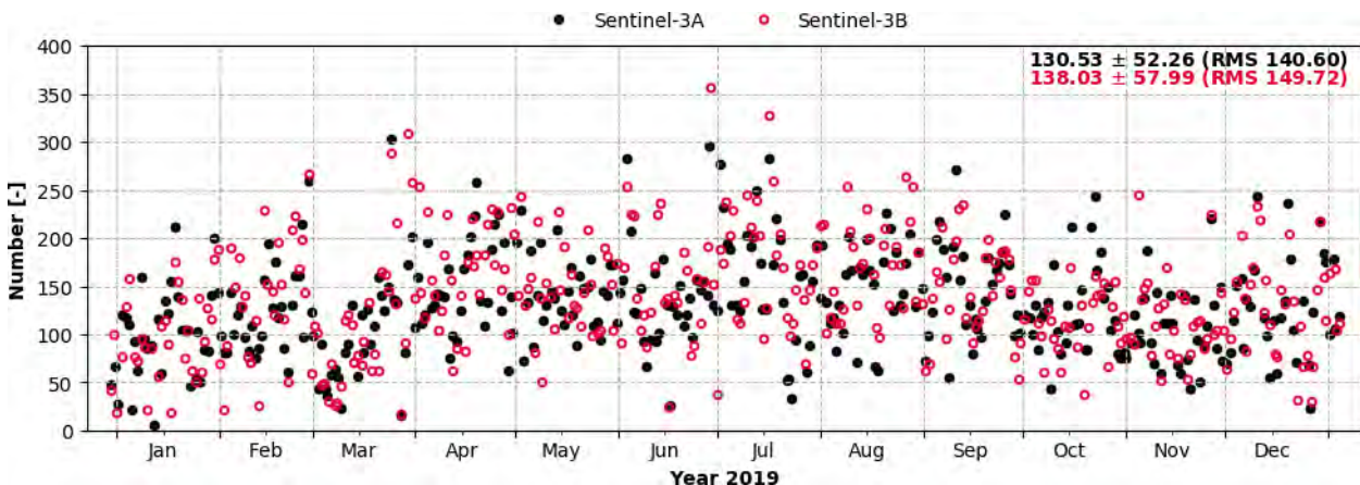
Figure 3-5: Daily total number of the accepted SLR observations of all SLR stations tracking Sentinel-3A and Sentinel-3B satellites in 2019
