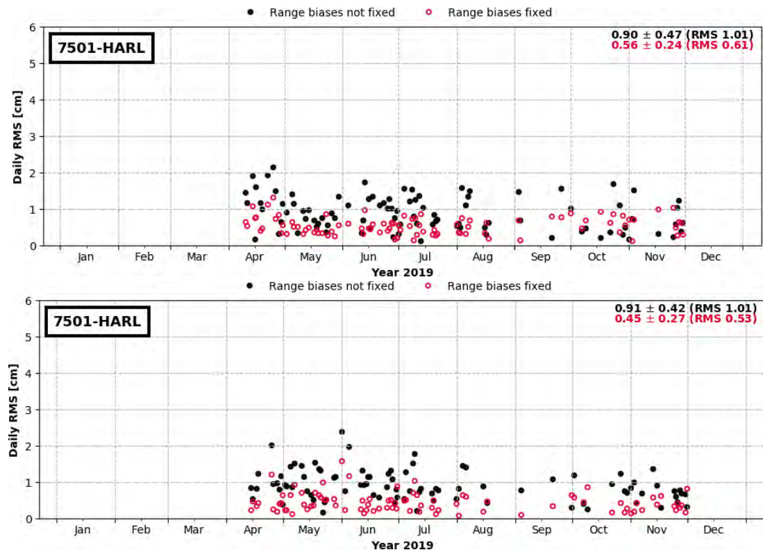
Figure 4-78: Daily RMS of the SLR observation residuals [1-range; cm] of the SLR station 7501 (HARL) in 2019 (above Sentinel-3A, and below Sentinel-3B)
