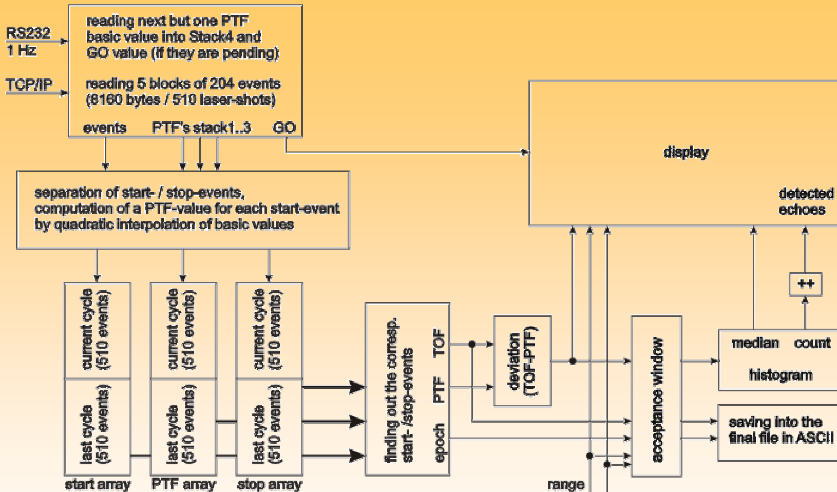
Scheme Of One Computation Cycle of Visualisation-PC (255 ms @ 2 kHz)
