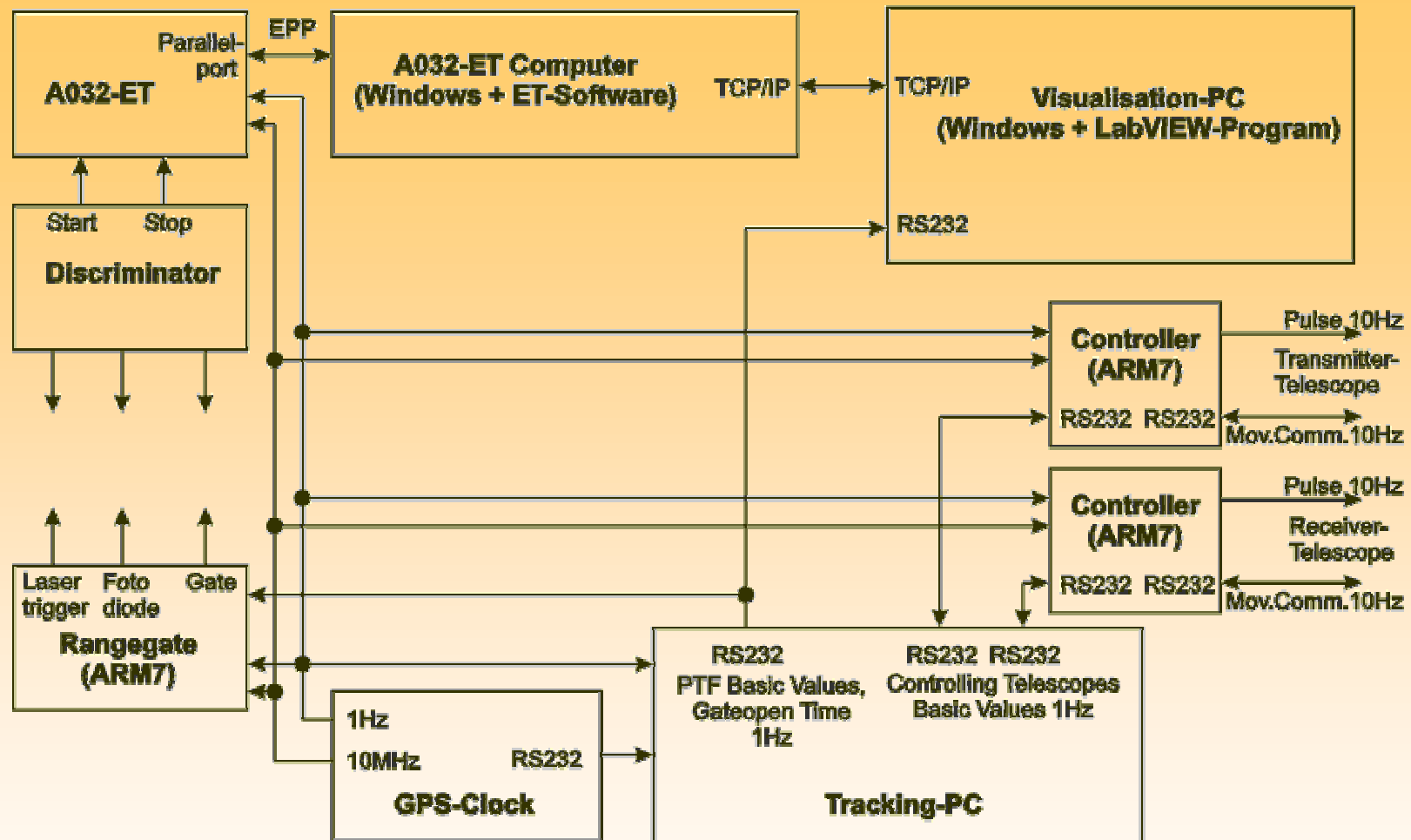
Scheme of KHz-SLR-Station at GFZ Potsdam
