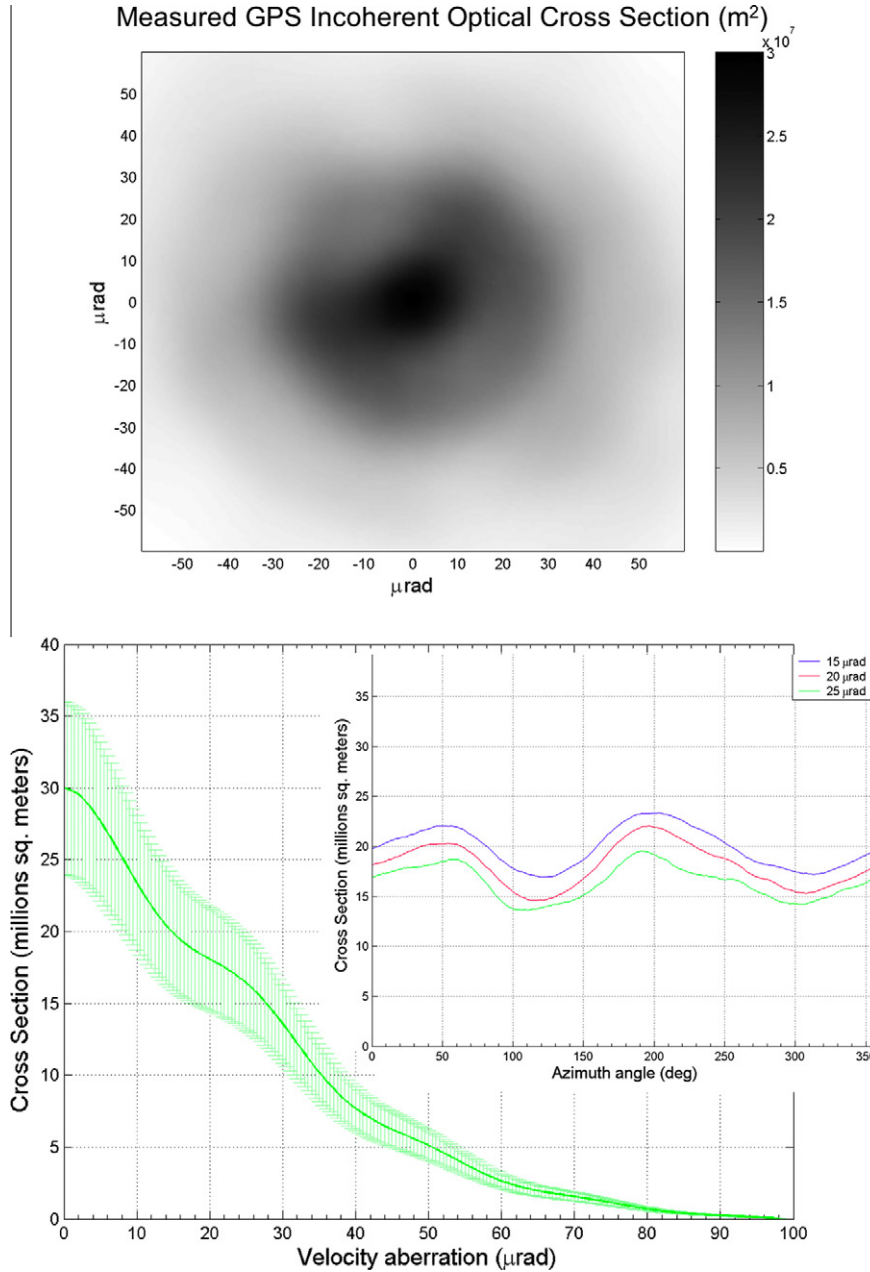
Fig. 22. GPS incoherent on-axis optical cross section measured at 532 nm. Top plot: \sigma_{\text{GPS,inc,AIC},0} vs. \theta_x, \theta_y . Bottom plot: averaged \sigma_{\text{GPS,inc,AIC},0} vs. velocity aberration; inset: \sigma_{\text{GPS,inc,AIC},0} vs. azimuth counted anticlockwise from the \theta_x > 0 axis of the top plot.
