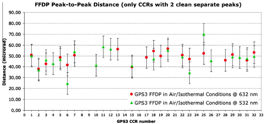
Fig. 20. FFDPs of the GPS flight retroreflectors with two clean separate peaks taken at 632 and 532 nm in air and isothermal conditions. The nominal distance is \sim 50 \mu\text{rad} .
