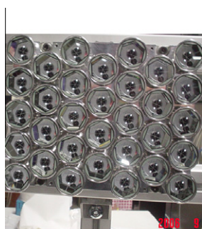
Fig. 2. Left: the third GPS flight CCR array SCF-Tested at LNF. Right: GPS/GIOVE laser returns recorded by the ILRS station at Graz, Austria (courtesy of G. Kirchner).
