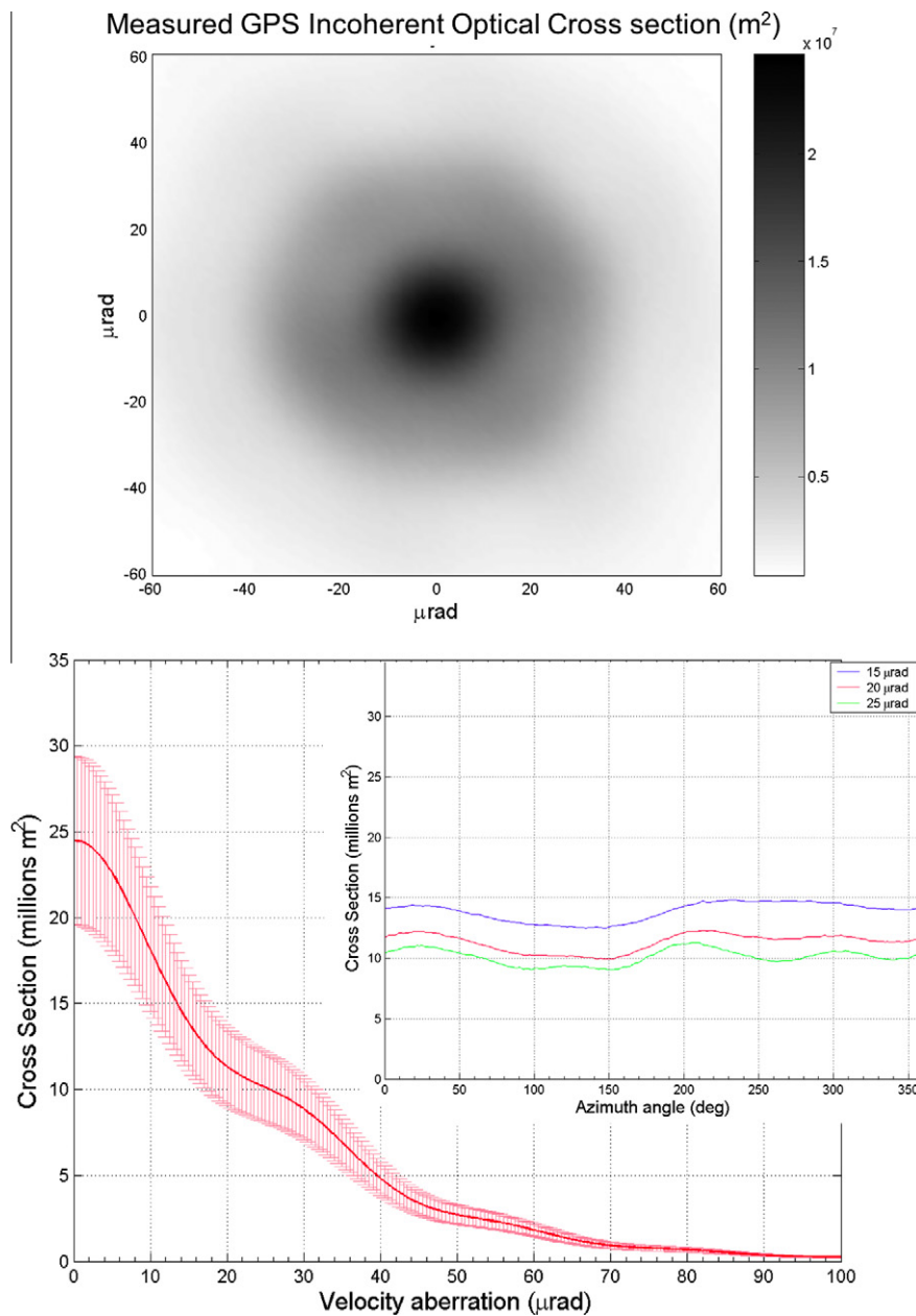
Fig. 21. GPS incoherent on-axis optical cross section measured at 632 nm. Top plot: \sigma_{\text{GPS},inc,AIC,0} vs. \theta_x, \theta_y . Bottom plot: averaged \sigma_{\text{GPS},inc,AIC,0} vs. velocity aberration; inset: \sigma_{\text{GPS},inc,AIC,0} vs. azimuth counted anticlockwise from the \theta_x > 0 axis of the top plot.
