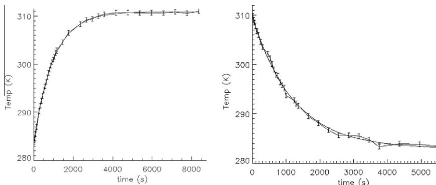
Fig. 14. CCR exponential heating (left) and cooling (right) curves with SS turned on and turned off: \tau_{CCR} = (1100 \pm 100) s, \Delta T = (28 \pm 1) K.
