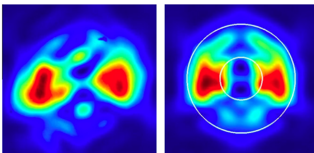
Fig. 6. Measured LAGEOS FFDP (left) and FFDP modeled with \text{DAO} \sim 1.25'' (the white circles show the radius of FFDP maxima for \text{DAO} = 0.75'' and 1.75'' ).
